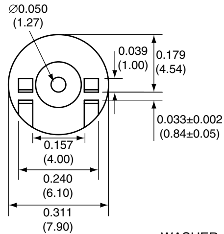
WASHER
