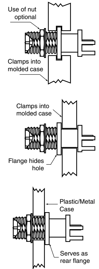
MOUNTING METHODS
