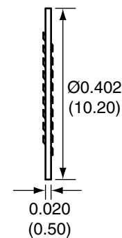
WASHER
